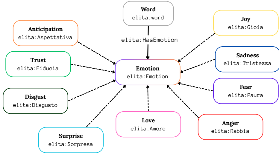
Figure 2: elita ontology
